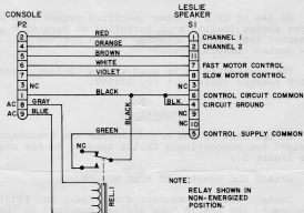
Figure 2. Schematic, Adapter 138851
